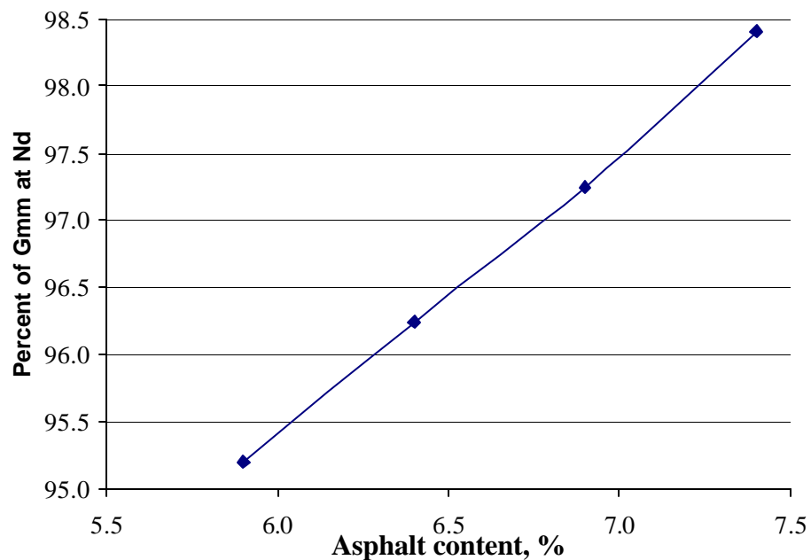
Figure C.11 Asphalt content versus percent Gmm at Nd-Supeprave light traffic mix.
