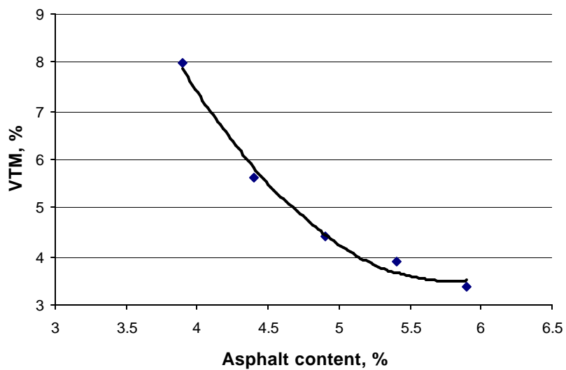
Figure B.4 Asphalt content versus VTM – Marshall heavy traffic mix
