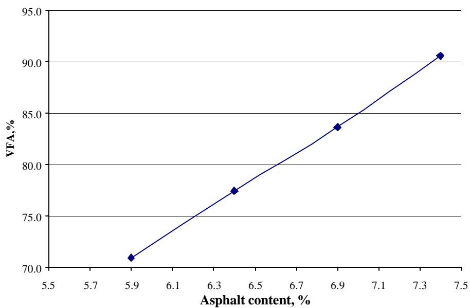
Figure C.12 Asphalt content versus VFA - Superpave light traffic level
