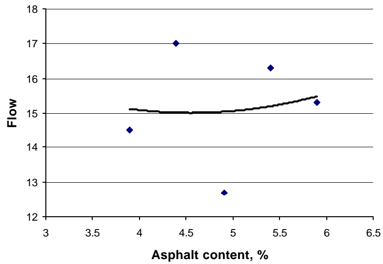
Figure B.3 Asphalt content versus Flow – Marshall heavy traffic mix
